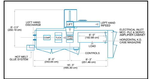
Sample machine layout
